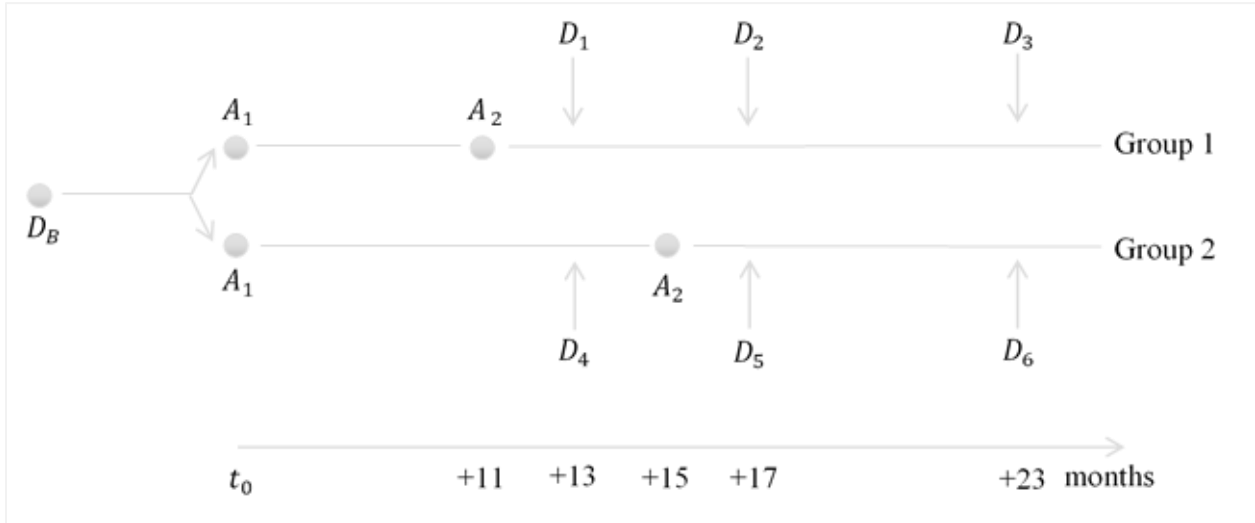
Figure 1 Identification Strategy
