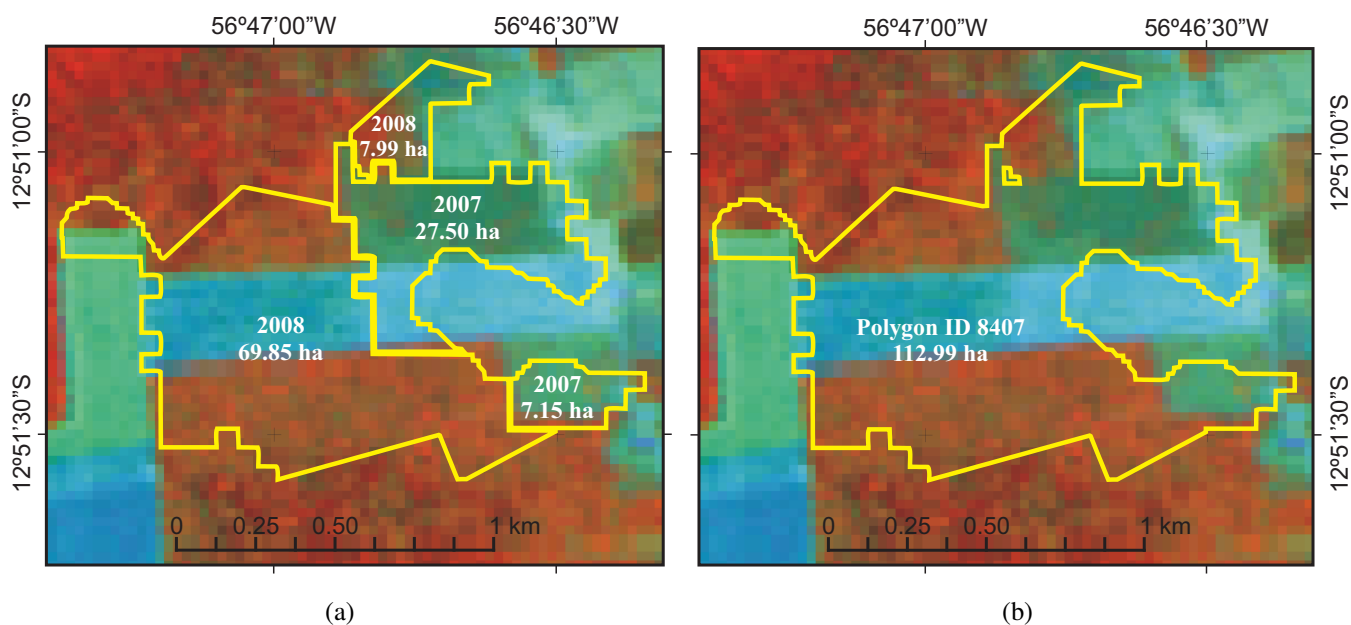
Figure 2. Example of the fusion of four PRODES polygons. Without fusion (a), two polygons would not be monitored because they measure less than 25 ha. After fusion (b) a single polygon was formed with an area greater than 25 ha.
